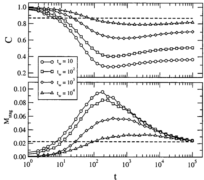
FIG. 8. Correlations and zero-field cooled magnetization in a staggered field in the SCIC model for N=10^5 , T=0.3 and different waiting times t_w = 10, 100, 1000, 10000 . The horizontal lines indicate the equilibrium values (42) and (43).
