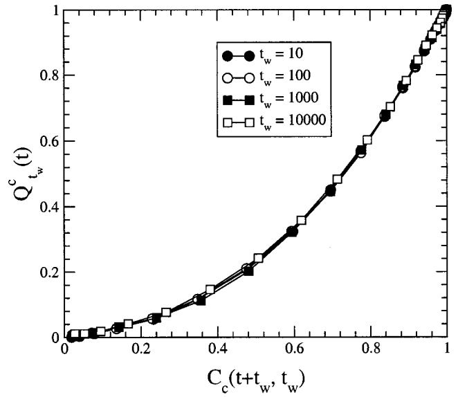
FIG. 12. Q_{t_w}^c(t) vs C_c(t+t_w, t_w) in the SCIC at T=0.11 .
