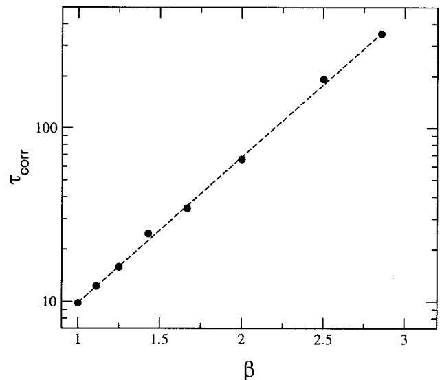
FIG. 6. Correlation time in the SCIC computed using Eq. (37) and fitted with an Arrhenius behavior. The best fit gives \tau_{\text{corr}} = 1.43 \exp(1.93\beta) .
