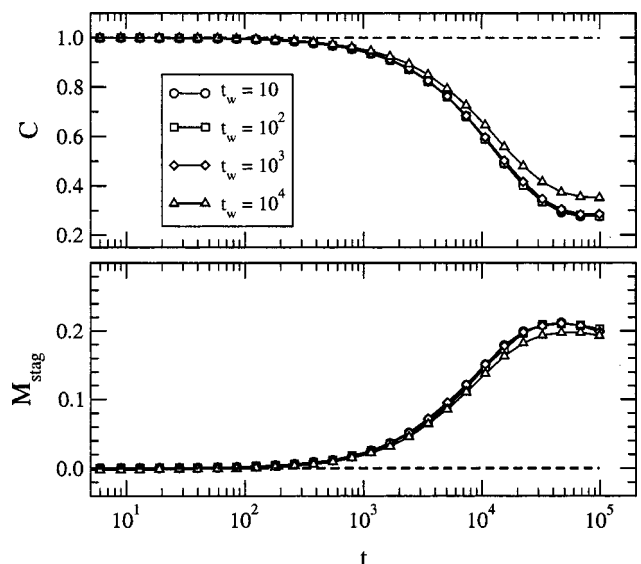
FIG. 9. Correlations and zero-field cooled magnetization in a staggered field in the SCIC model for N=10^5 , T=0.11 and different waiting times t_w = 10, 100, 1000, 10000 . The horizontal lines indicate the equilibrium values (43).
