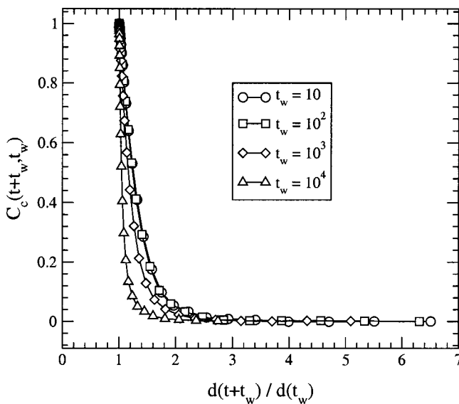
FIG. 14. Connected correlations C_c(t+t_w, t_w) (34) in the SCIC for N=10^5 , T=0.15 plotted vs d(t+t_w)/d(t_w) .
