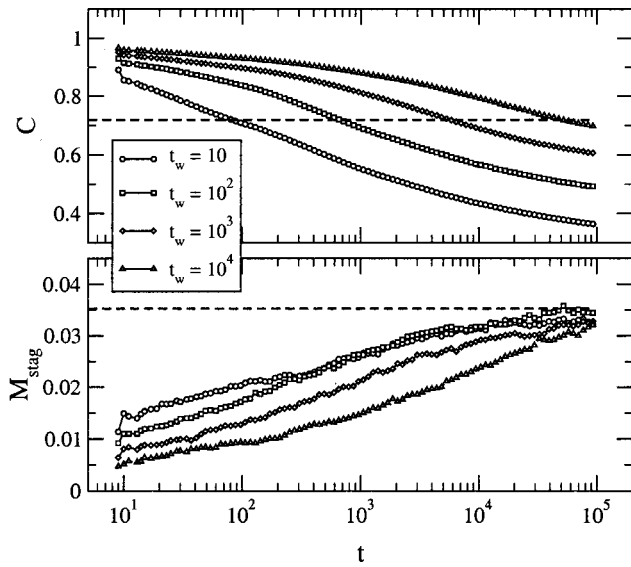
FIG. 16. Correlations and zero-field cooled magnetization in a staggered field in the ACIC model for N=10^5 , T=0.4 and different waiting times t_w=10,100,1\,000,10\,000 . The horizontal line indicates the equilibrium value (43).
