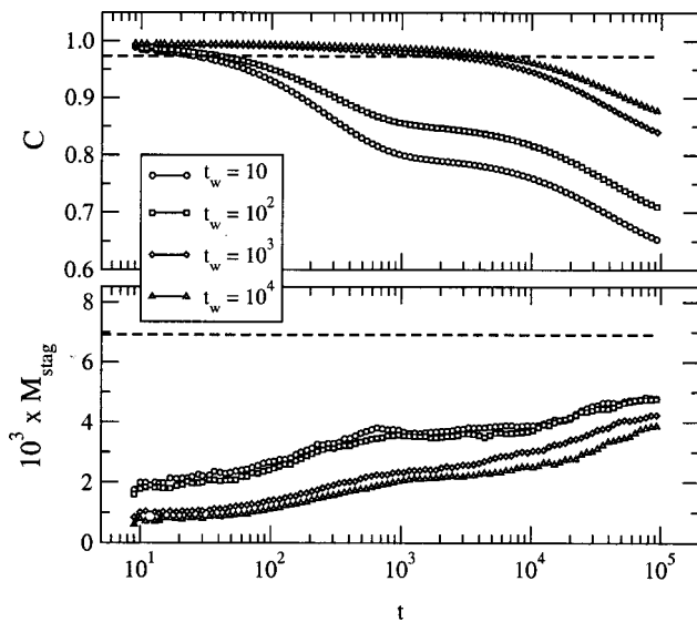
FIG. 17. Correlations and zero-field cooled magnetization in a staggered field in the ACIC model for N=10^5 , T=0.2 and different waiting times t_w=10,100,1\,000,10\,000 . The horizontal line indicates the equilibrium value (43).
