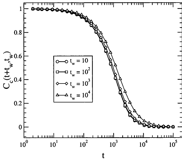
FIG. 13. Connected correlations C_c(t+t_w, t_w) in the SCIC for N=10^5 , T=0.15 and different waiting times t_w=10, 100, 1000, 10000 . Aging is present for times larger than \tau_1 = \exp(\beta) .
